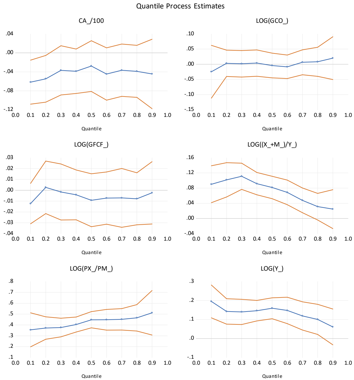
Figure 17: Quantile estimates
